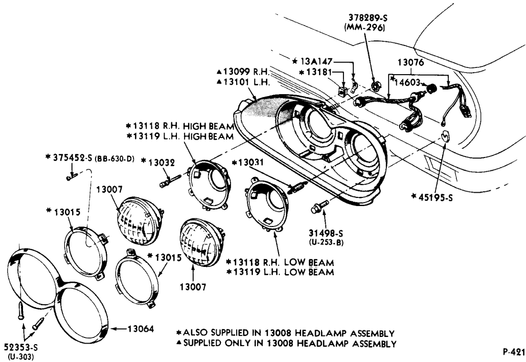
HEADLAMP PARTS 1965 THUNDERBIRD
