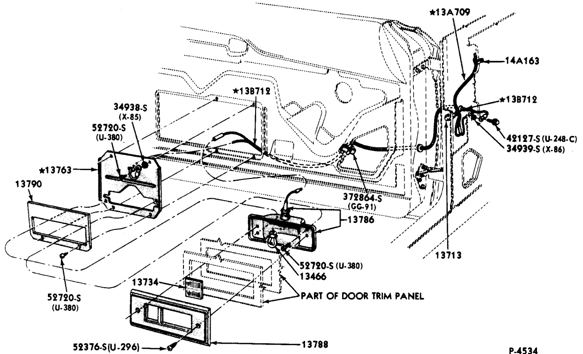
COURTESY LAMPS and WIRING - INTERIOR DOOR 1965 FAIRLANE
