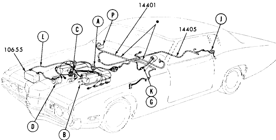
IGNITION, STARTING, CHARGING GAUGES WIRING SYSTEMS
