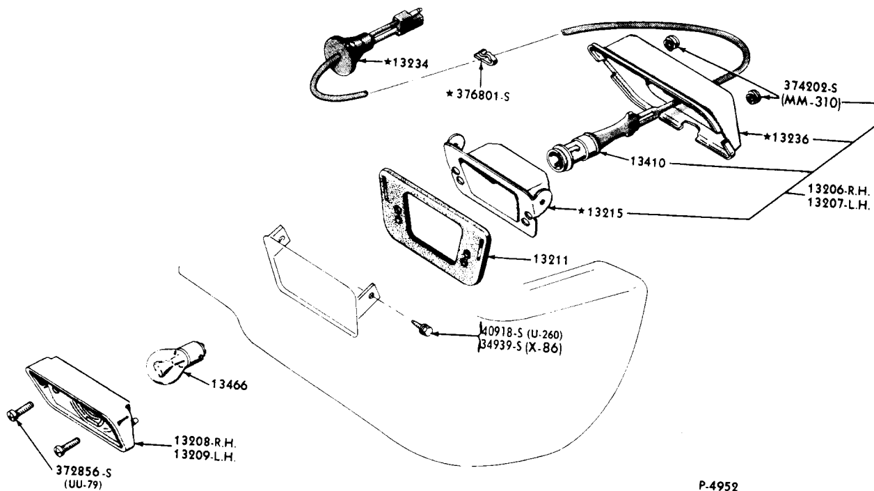
PARKING LAMP - TYPICAL 1966/67 FAIRLANE 1966/67 FALCON
