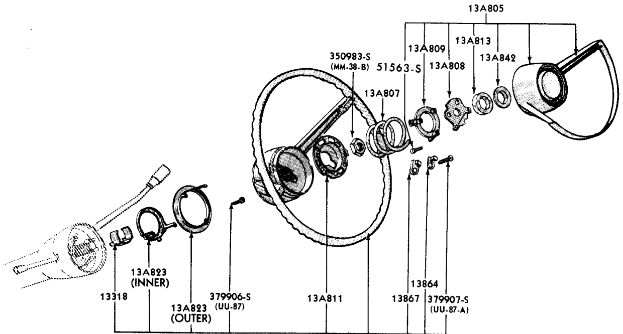
HORN RING, STEERING WHEEL and RELATED PARTS 1966/72 BRONCO
