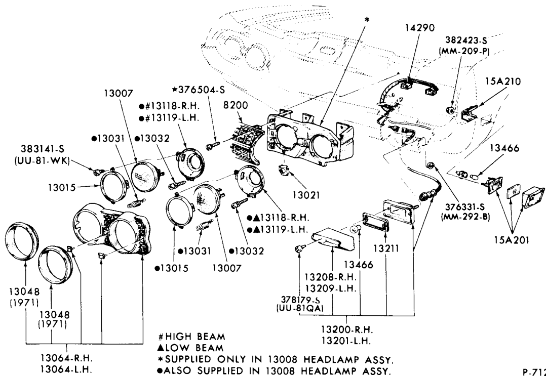
HEADLAMP, PARKING LAMP, FENDER SIDE MARKER LAMP and RELATED PARTS 1970/71 FAIRLANE - BODY TYPES 54A, B, 62A, 63H, 65A, B, 66A, 71B, D 1970 FAIRLANE BODY TYPE 66B - "BEFORE 12/30/69"
