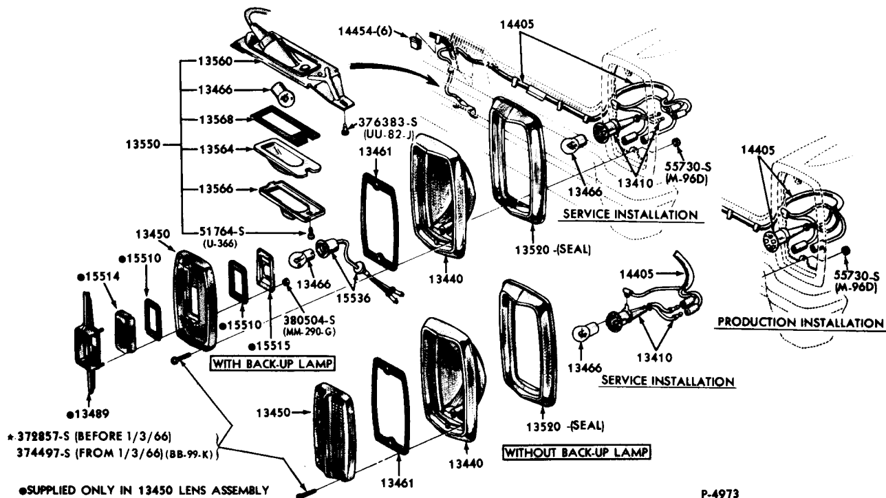
REAR LAMP, BACK UP LAMP and LICENSE PLATE LAMP 1966 FAIRLANE - except STATION WAGON
