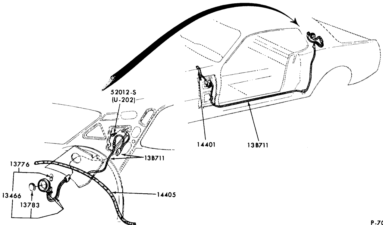
COURTESY LAMP and RELATED PARTS - PILLAR MOUNTED 1969/72 MUSTANG
