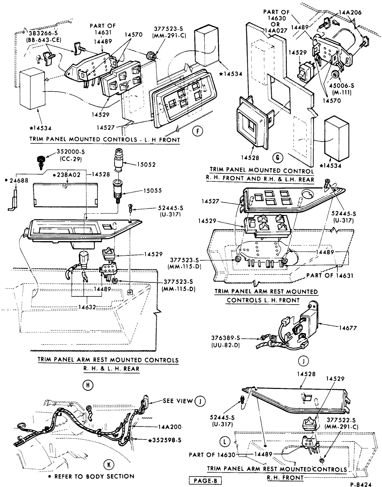
ELECTRIC WINDOW REGULATORS, CONTROLS, WIRING SYSTEM - PAGE B 1971/72 FORD
