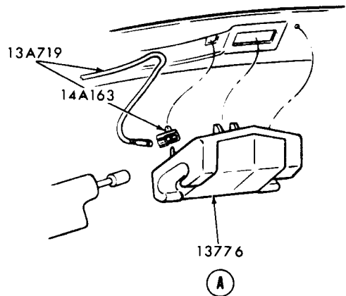
MAP LAMPS and WIRING - ROOF CONSOLE 1967/68 MUSTANG
