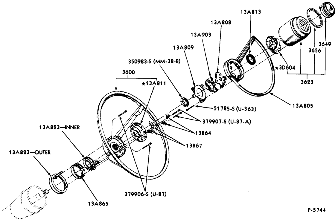
HORN RING, STEERING WHEEL and RELATED PARTS -- NON - WOODGRAIN WHEEL 1967 FORD
