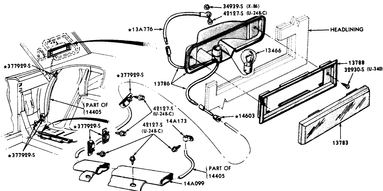
PILLAR LAMP and RELATED PARTS 1965/66 THUNDERBIRD - BODY TYPE 63A
