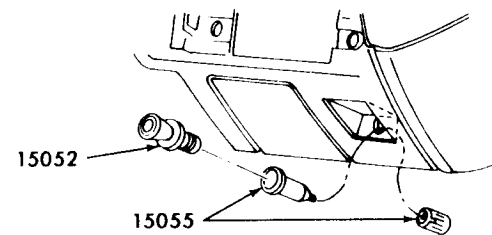
CIGAR LIGHTER INSTALLATION
