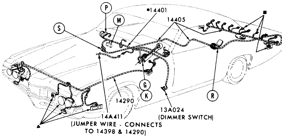
EXTERIOR LAMP WIRING SYSTEM
