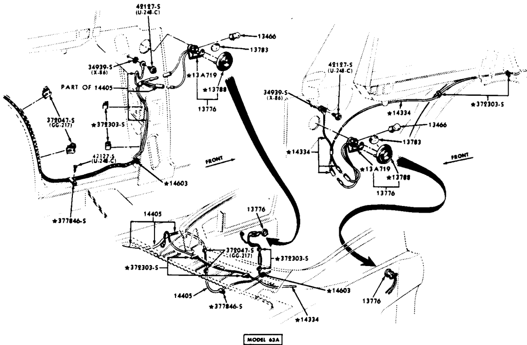
COURTESY LAMP and WIRING - INTERIOR QUARTER PANEL 1965/70 MUSTANG - "FASTBACK"
