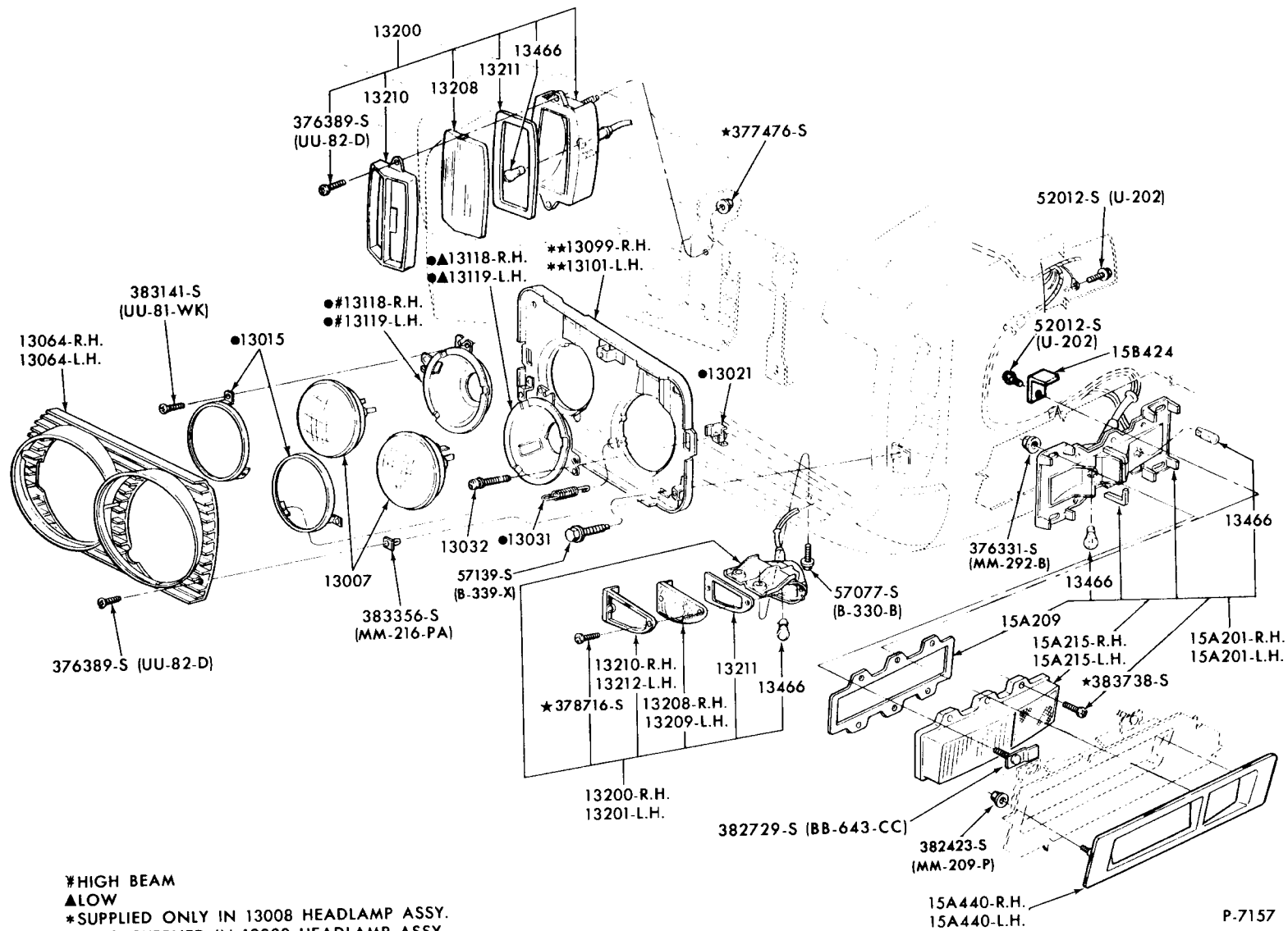
HEADLAMP, PARKING LAMP, FENDER SIDE MARKER LAMP and RELATED PARTS 1970/71 THUNDERBIRD
