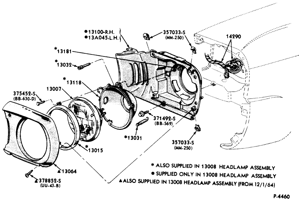
HEADLAMP PARTS 1965/66 MUSTANG
