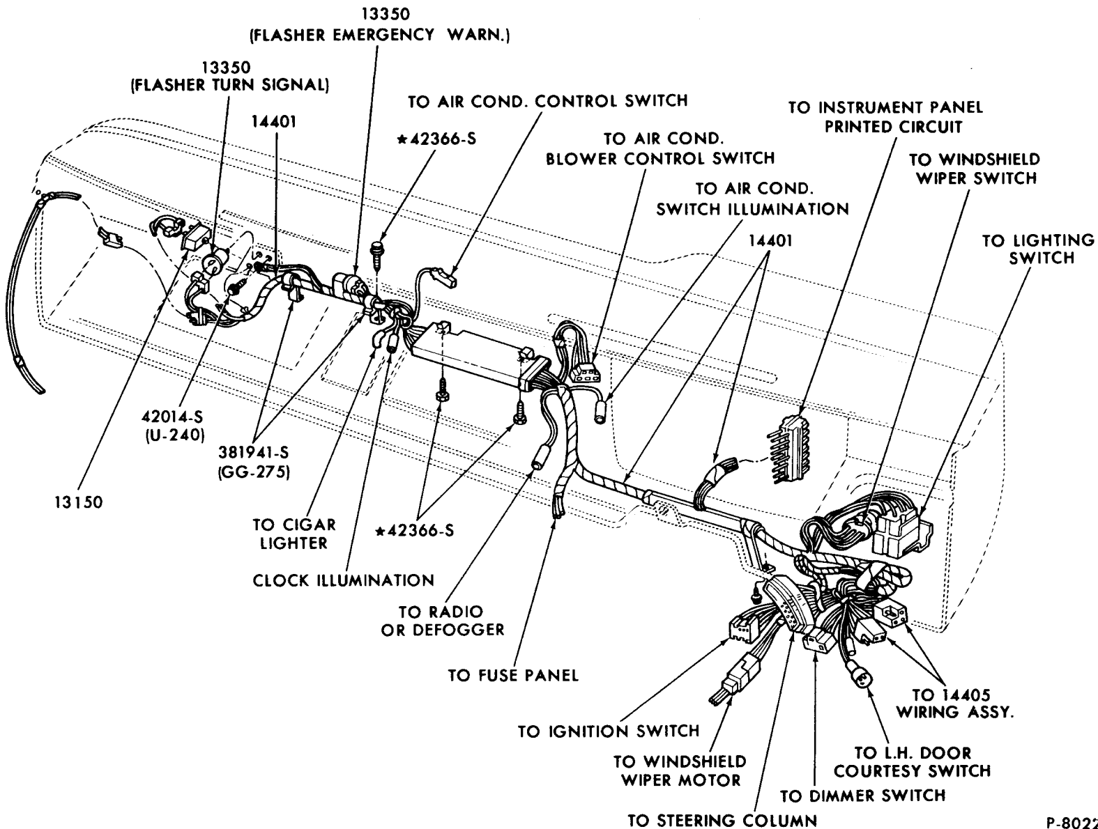
WIRING INSTRUMENT PANEL
