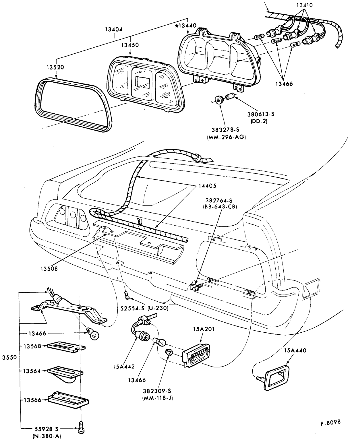
REAR LAMP, BACK UP LAMP, LICENSE PLATE LAMP and BODY SIDE MARKER LAMP 1971/72 MUSTANG
