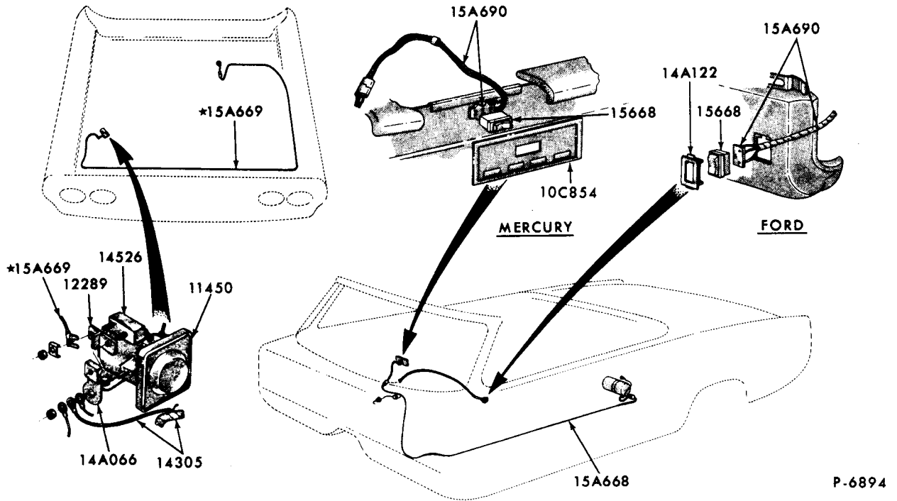
CONVERTIBLE TOP ELECTRICAL SYSTEM 1969/70 FORD
