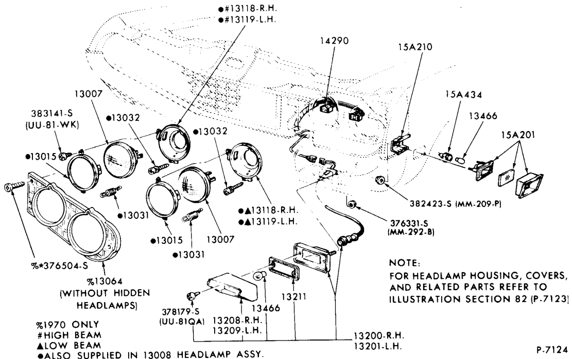
HEADLAMP, PARKING LAMP, FENDER SIDE MARKER LAMP and RELATED PARTS 1970 FAIRLANE/TORINO BODY TYPE 66B - "FROM 12/30/69" 1970 FAIRLANE/TORINO - BODY TYPES 54C, 57C, E, 63F, 65C, E, 66C, E, 71C, E, 76 (WITH & WITHOUT HEADLAMP COVERS) 1971 TORINO - BODY TYPES 54C, 57C, E, 63C, F, 65C, E, 66B, C, E, 71C, E, 76F (WITH HEADLAMP COVERS)
