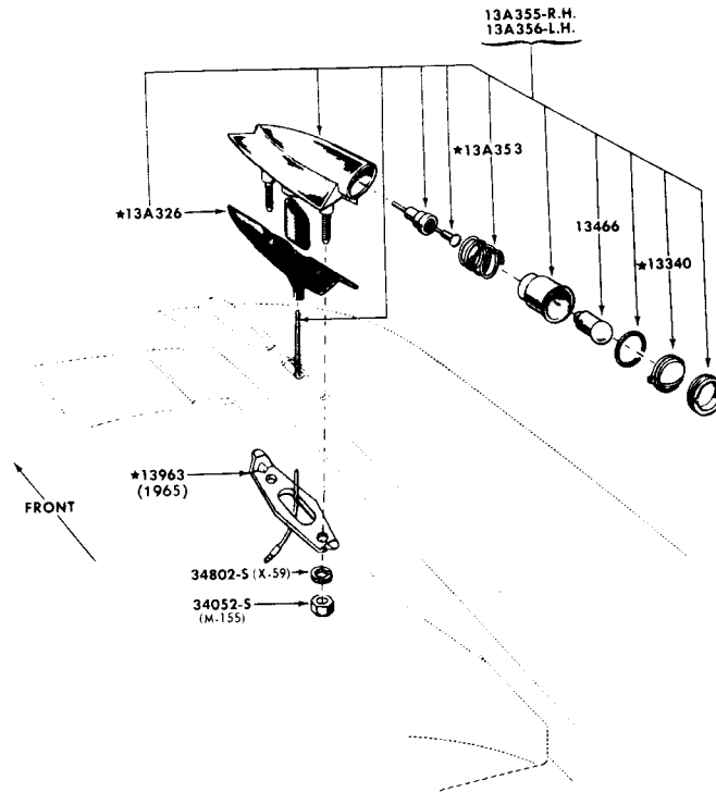
TURN INDICATOR LAMP - FENDER MOUNTED 1965/66 THUNDERBIRD
