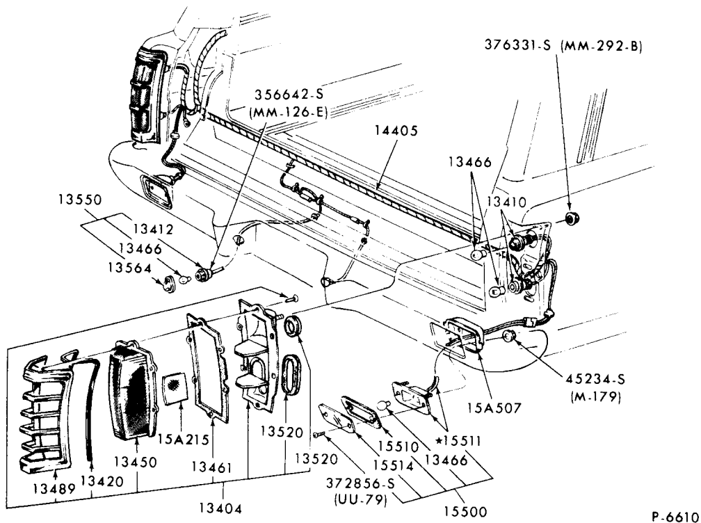
REAR LAMP, BACK UP LAMP & LICENSE PLATE LAMP 1969/70 FORD - STATION WAGON
