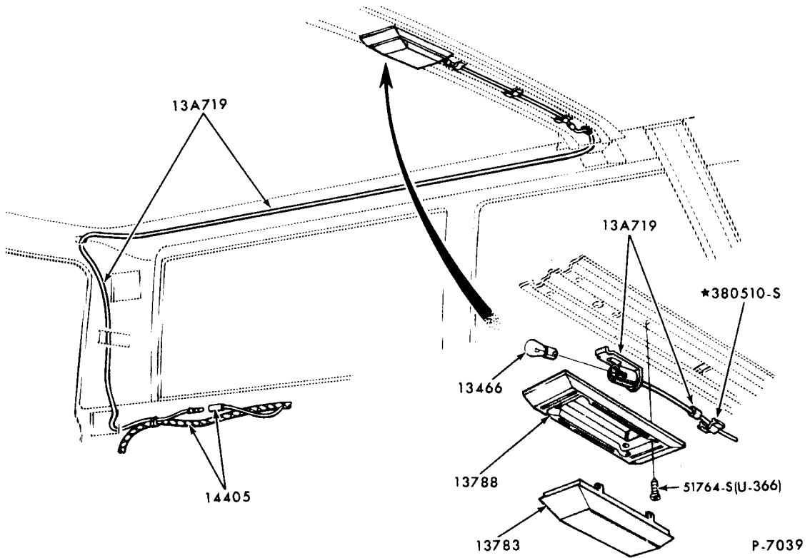
DOMELAMP and RELATED PARTS 1966/72 FORD and 1971/72 TORINO
