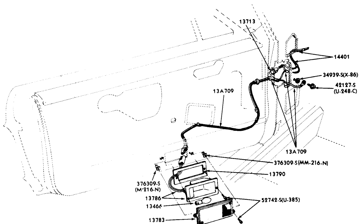
COURTESY LAMP and WIRING - INTERIOR DOOR 1967/68 MUSTANG
