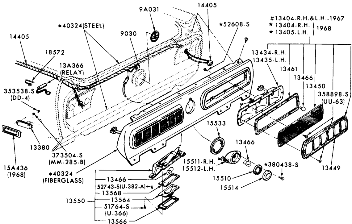
REAR LAMP, BACK UP LAMP and LICENSE PLATE LAMP 1967/68 MUSTANG - GT 350/500
