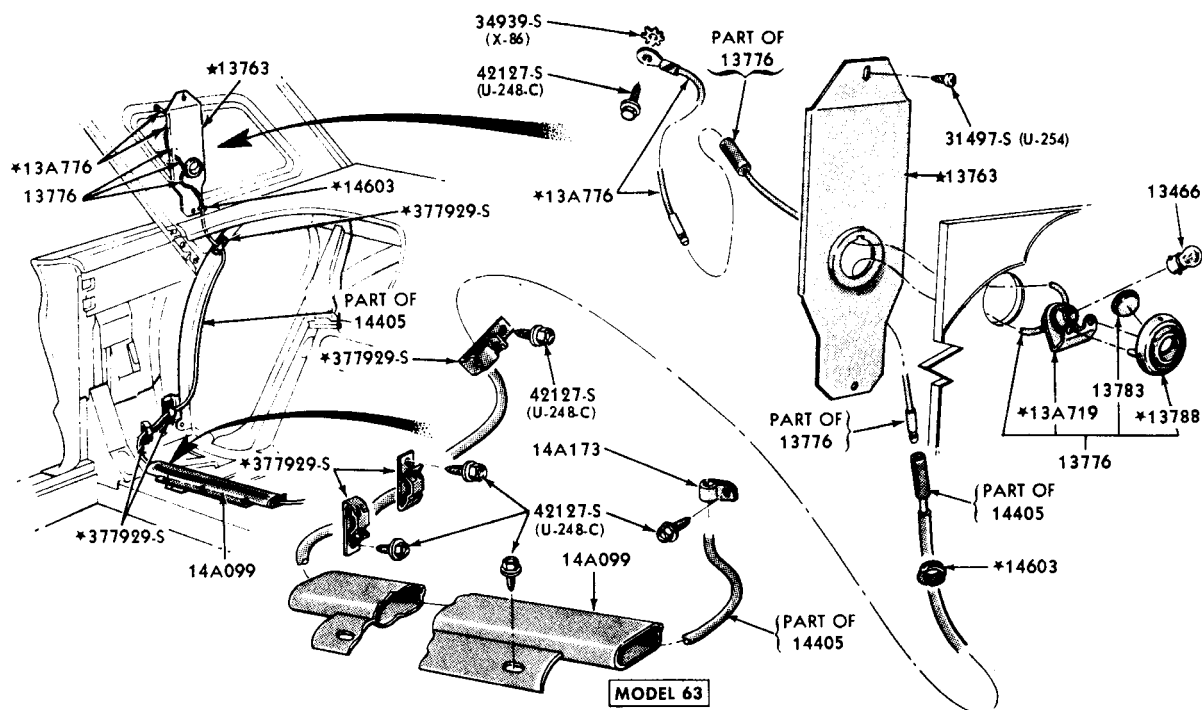
PILLAR LAMP and RELATED PARTS 1965/66 THUNDERBIRD - BODY TYPE 63A
