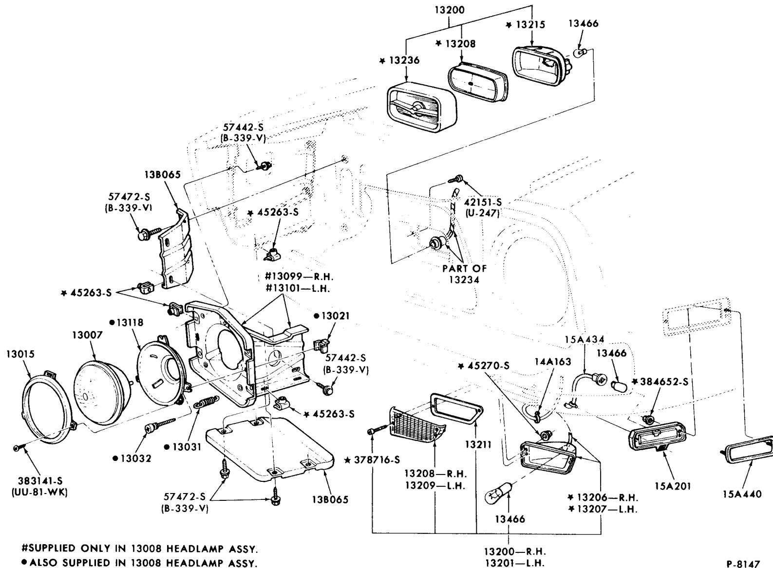
HEADLAMP, PARKING LAMP, FENDER SIDE MARKER LAMP and RELATED PARTS 1971/72 MUSTANG
