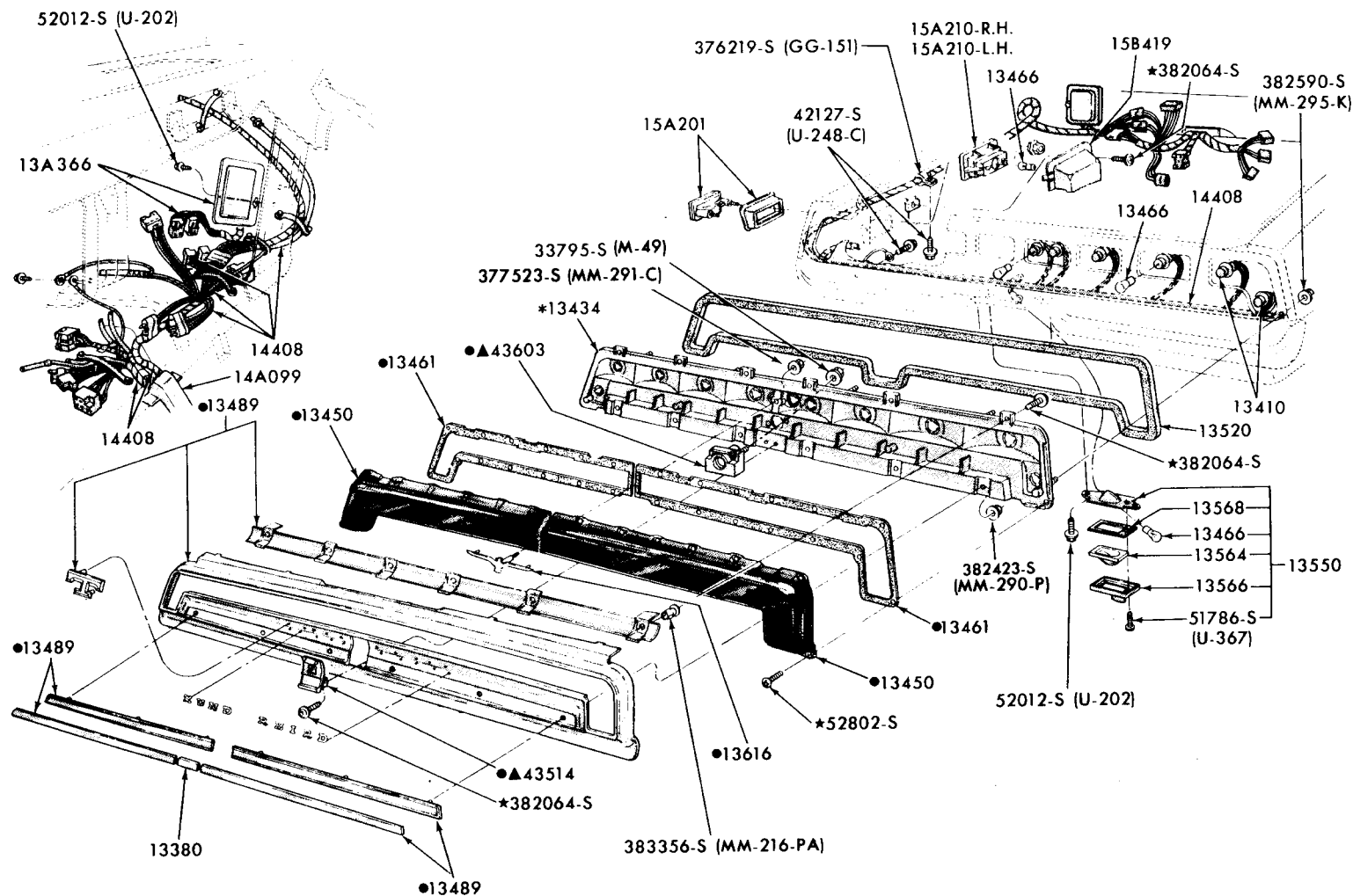
REAR LAMP, BACK UP LAMP, LICENSE PLATE LAMP and BODY SIDE MARKER LAMP 1970/71 THUNDERBIRD
