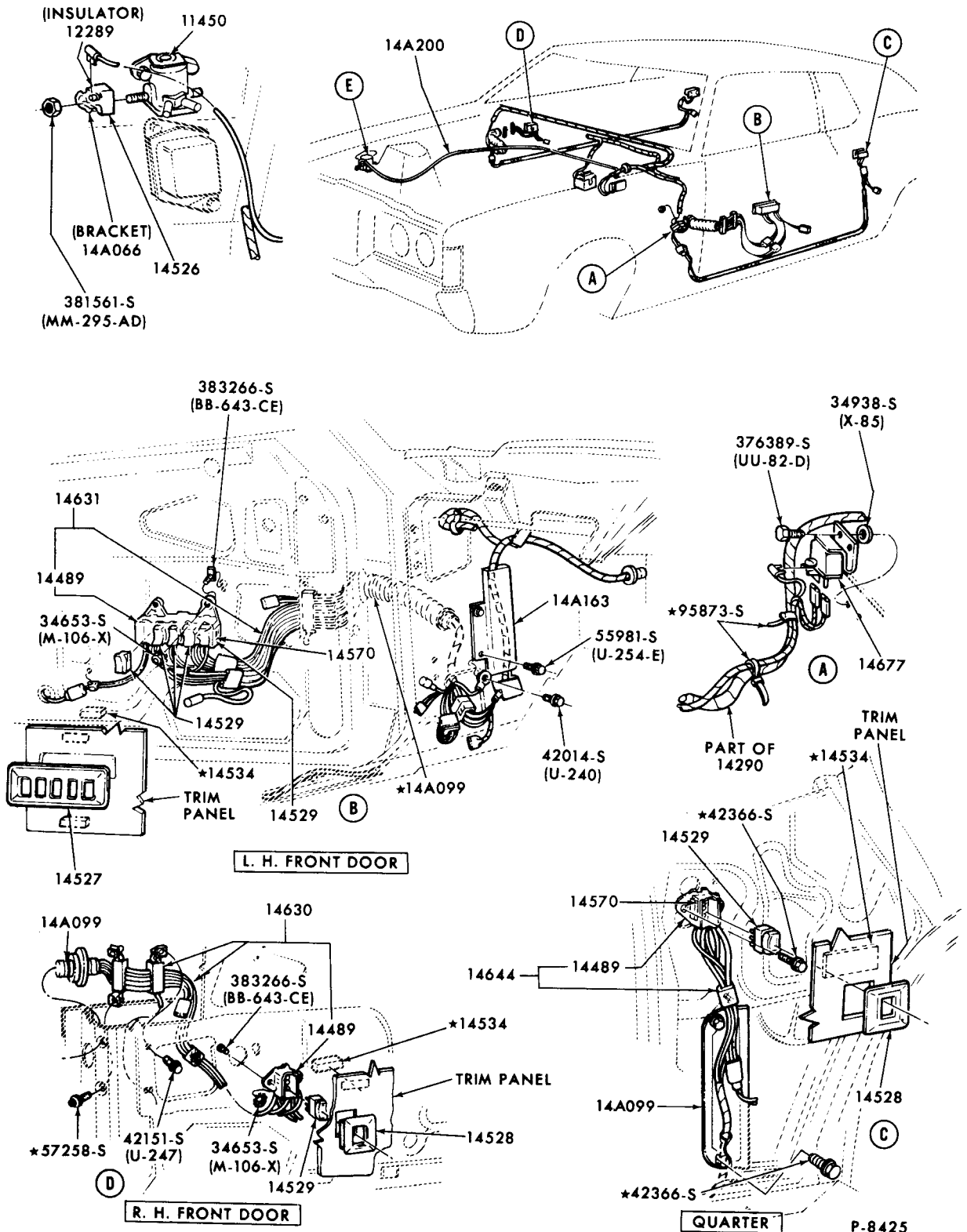
ELECTRIC WINDOW REGULATORS, CONTROLS, WIRING SYSTEM 1971/72 MUSTANG
