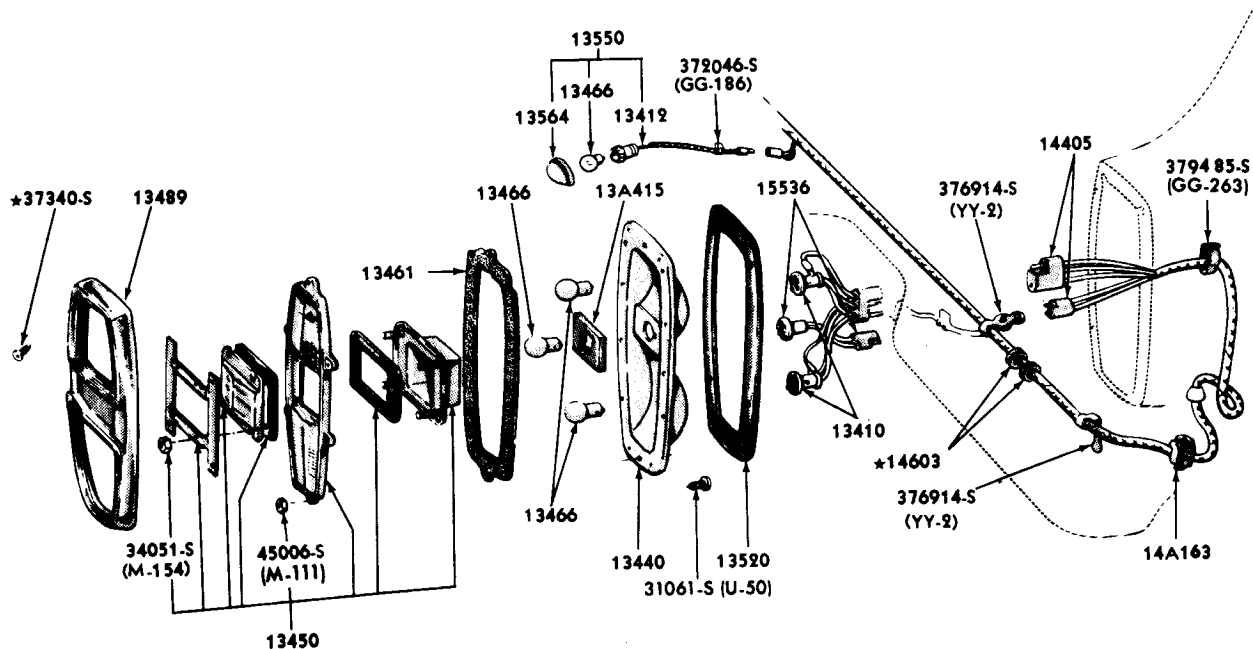
REAR LAMP, BACK UP LAMP and LICENSE PLATE LAMP 1967 FAIRLANE - except STATION WAGON and RANCHERO
