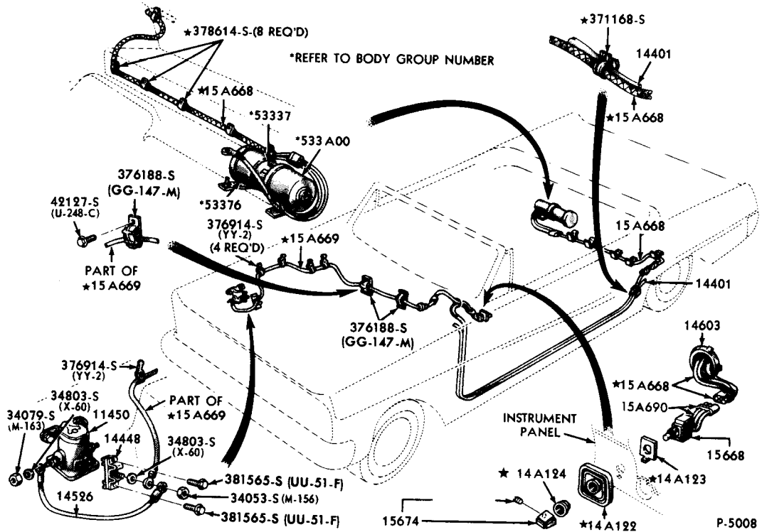
CONVERTIBLE TOP ELECTRICAL SYSTEM 1966/67 FAIRLANE
