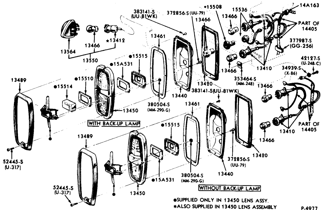
REAR LAMP, BACK UP LAMP and LICENSE PLATE LAMP 1966 FORD - STATION WAGON
