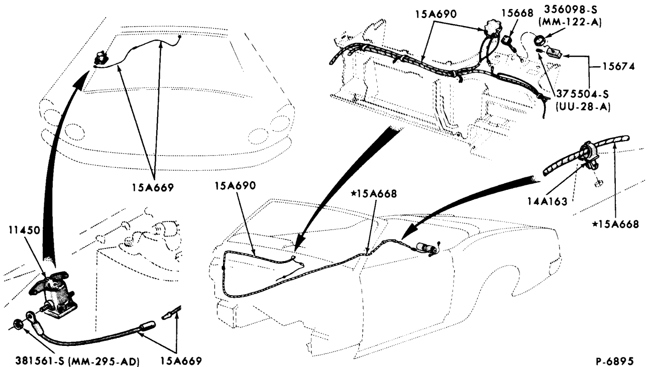
CONVERTIBLE TOP ELECTRICAL SYSTEM 1969/70 MUSTANG
