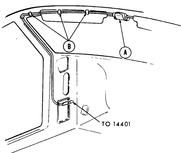
MAP LAMPS and WIRING - ROOF CONSOLE 1967/68 MUSTANG
