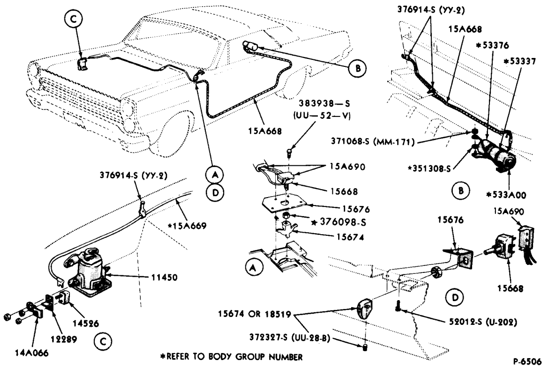
CONVERTIBLE TOP ELECTRICAL SYSTEM 1968/71 FAIRLANE/TORINO
