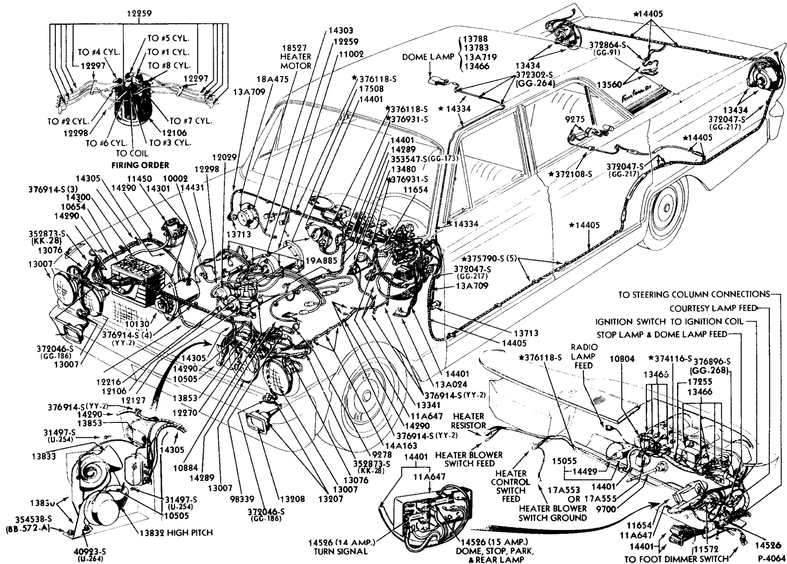
WIRING SYSTEM - "TYPICAL" 1965 FAIRLANE
